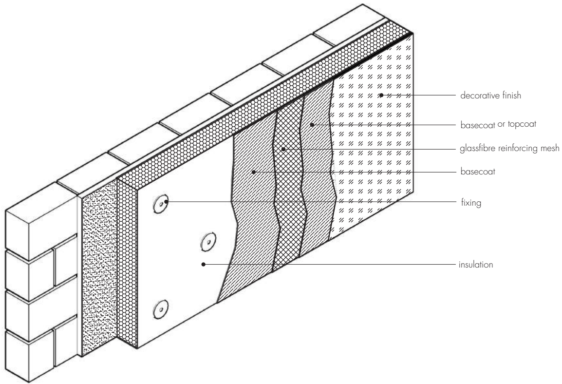
Figure 1 TERMOK8 Classico External Wall Insulation System
