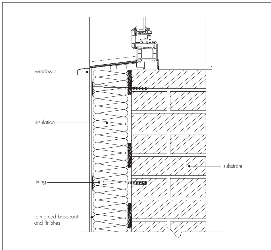
Figure 12 Window sill details
