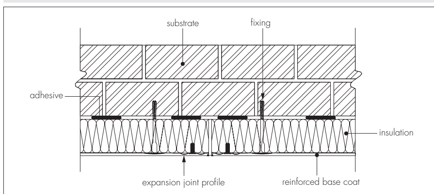
Figure 5 Typical movement joint
