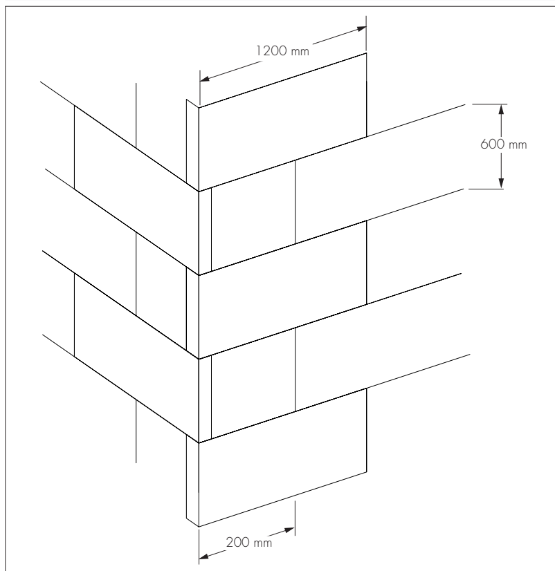
Figure 4 Typical arrangement of insulation boards
