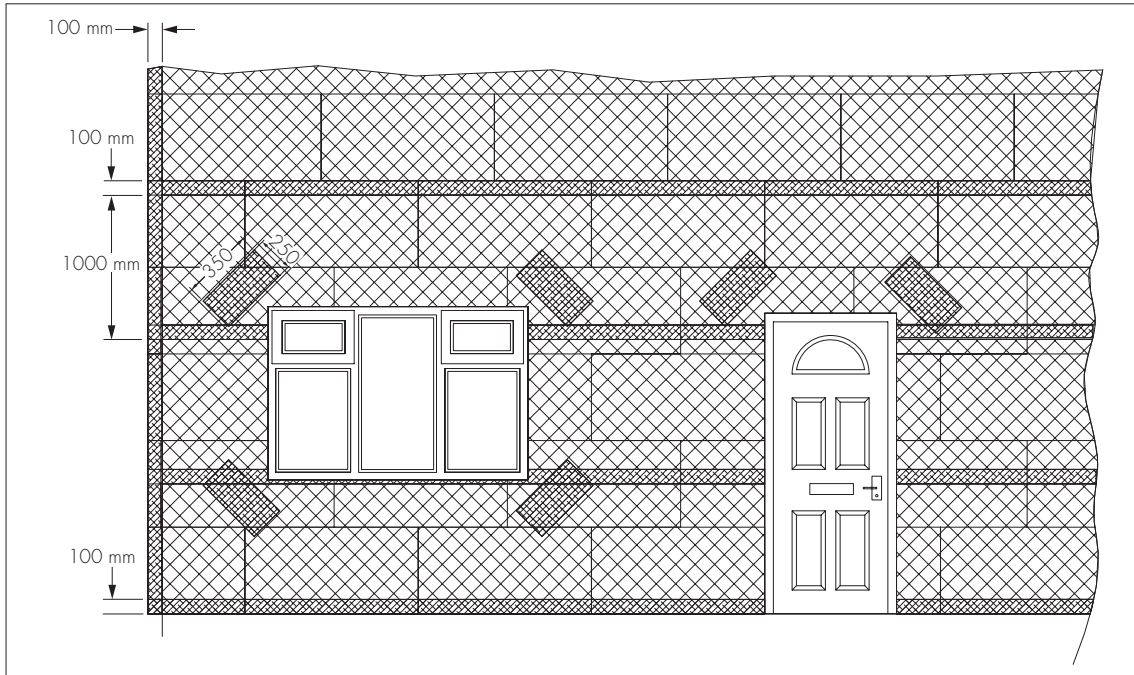
Figure 6 Reinforcement at openings
