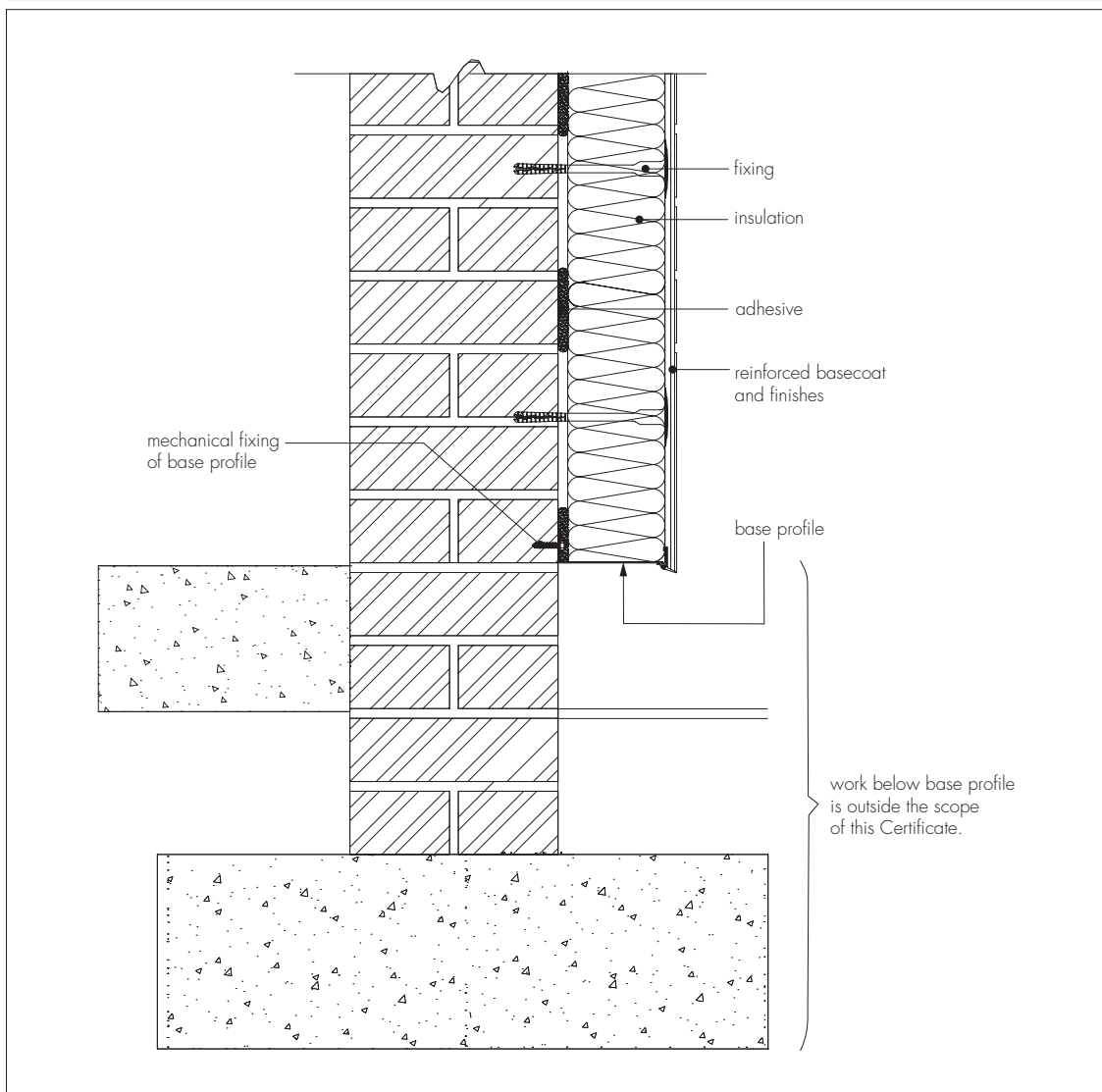
Figure 3 Typical section of base profile
