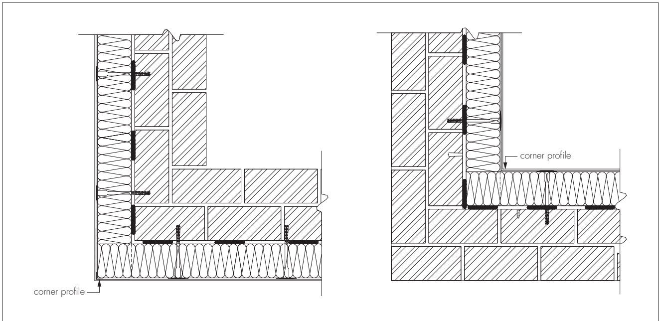
Figure 11 Corner details
