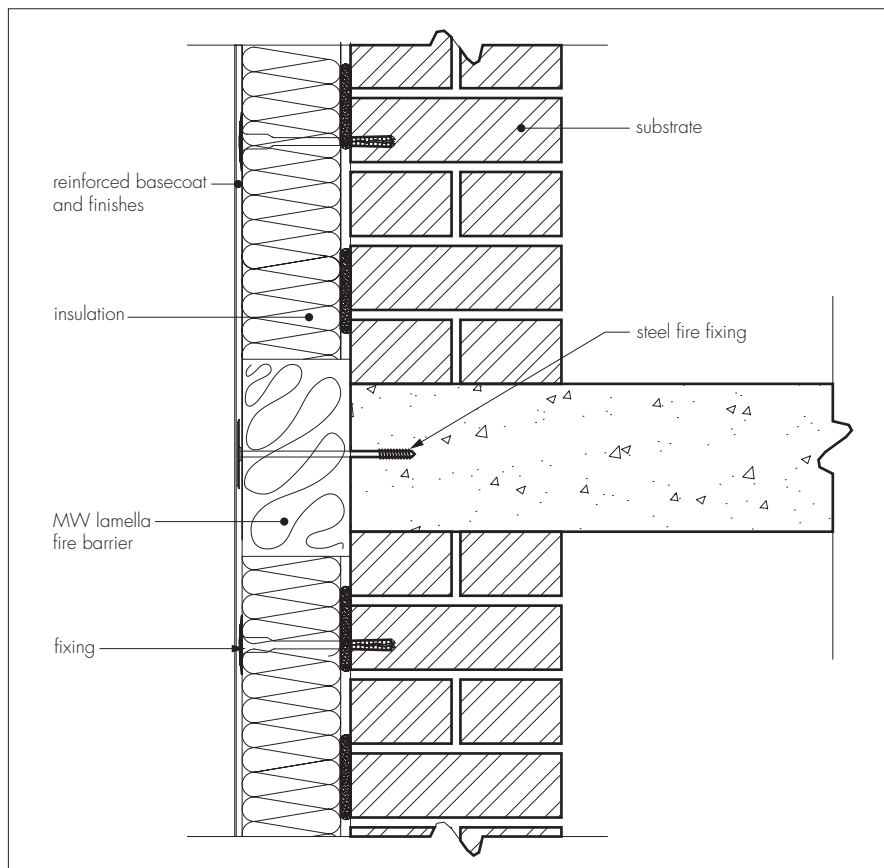
Figure 2 Fire barrier
