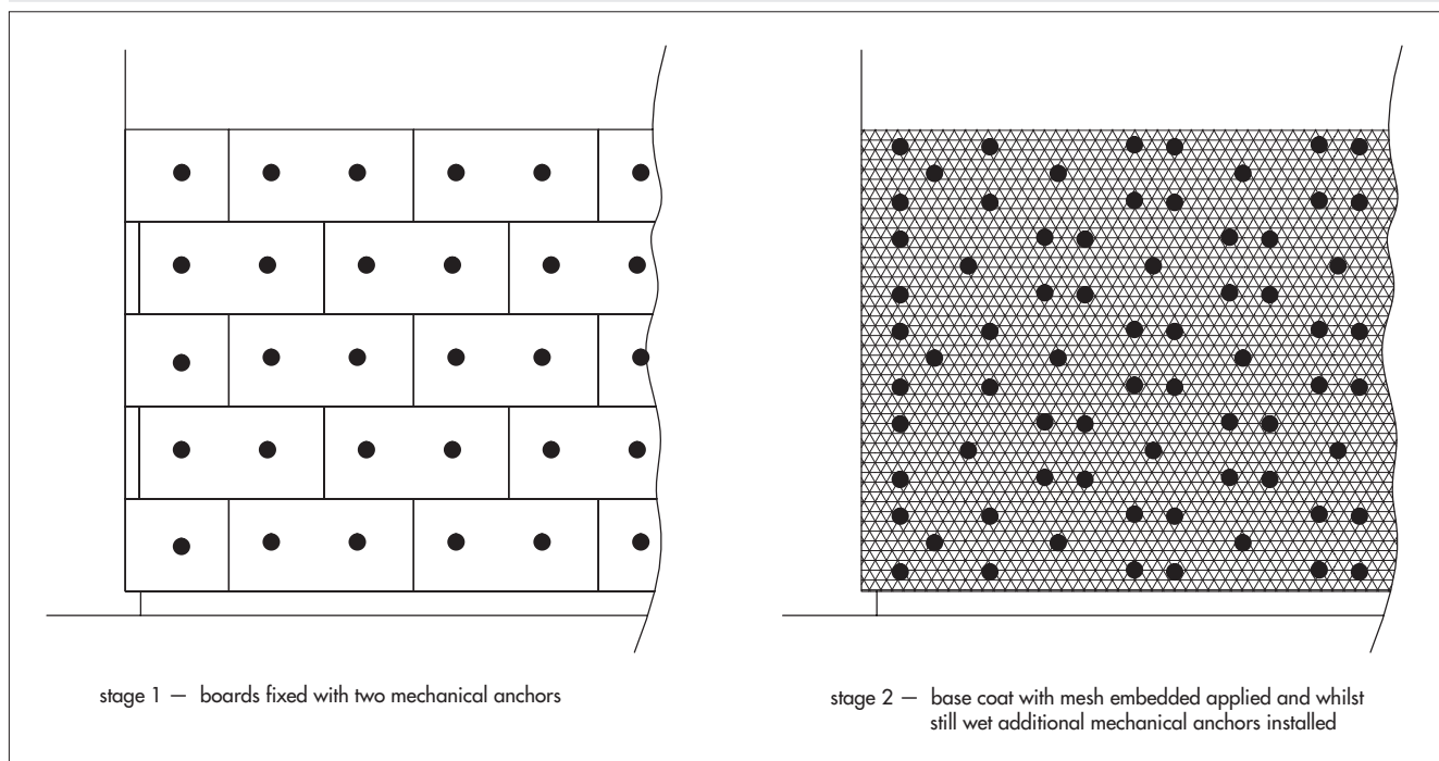
Figure 8 60-years durability fixings pattern
