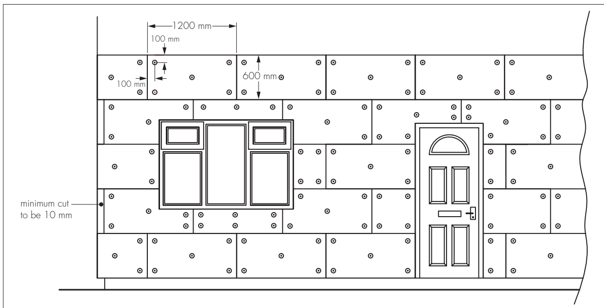
Figure 7 30-years durability fixings pattern
