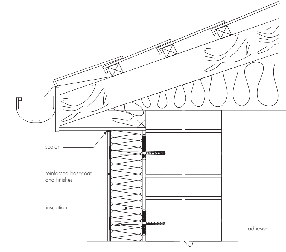
Figure 9 Typical roof eaves detail
