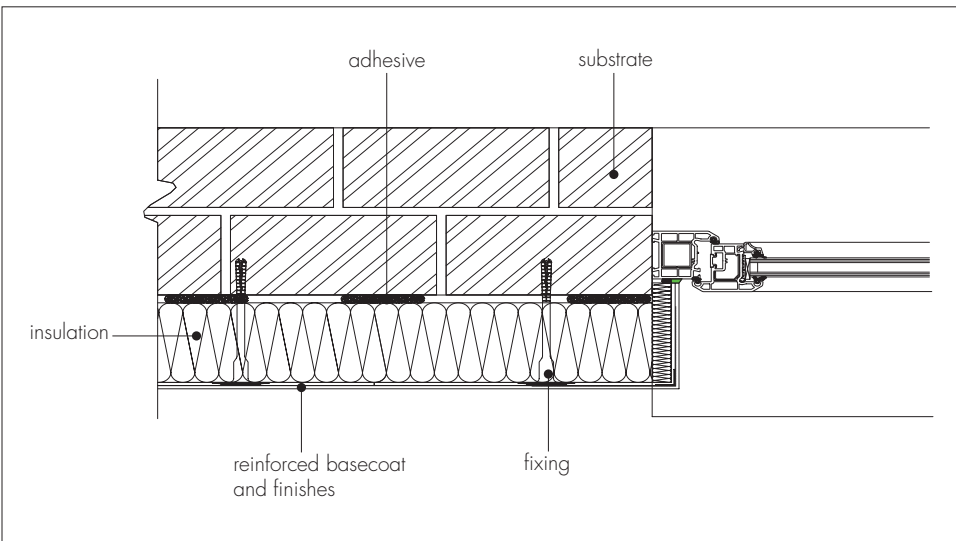
Figure 10 Window head details
